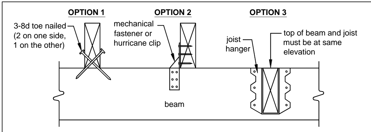
FIGURE 6: JOIST-TO-BEAM DETAIL
