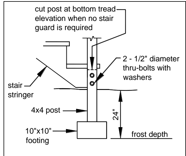
FIGURE 36: STAIR FOOTING DETAIL 42 inches deep not 24 inches
